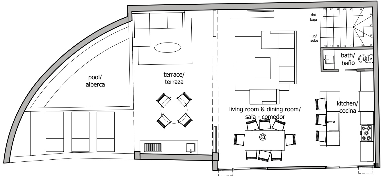
KEY PLAN
